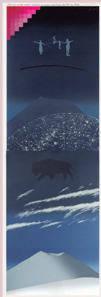
The Rise of the Earth's Shadow at Sunset Seen from the Pic du Midi, 1984.
